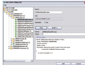
MIB Compiler
